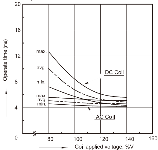
Operate time
