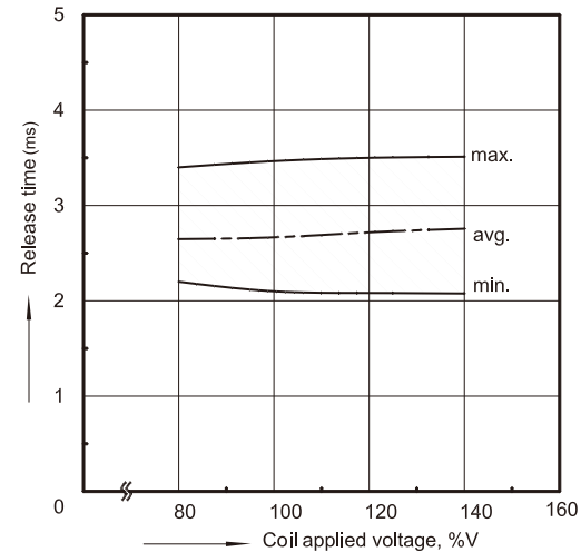
Release time
