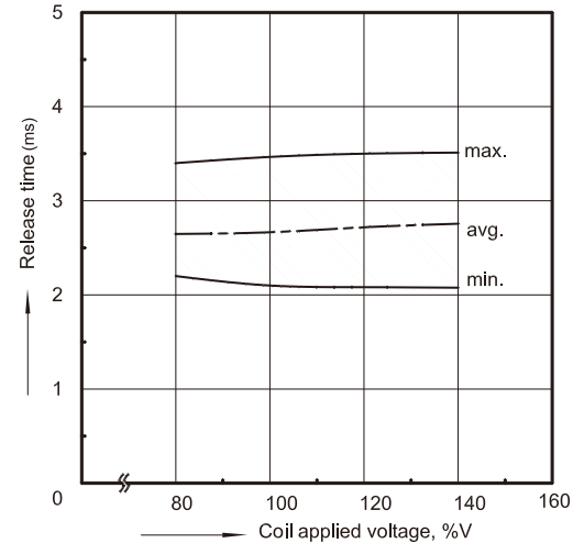
Release time
